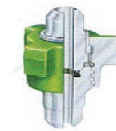
Fig 2002 Hammer Union 20,000 psi (1380 bar) cold working pressure
