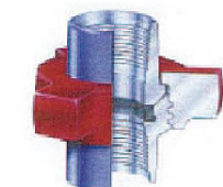
Fig 2002 Hammer Union 20,000 psi (1380 bar) cold working pressure
