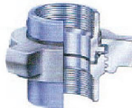
Fig 602 Hammer Union 6,000 psi (414 bar) cold working pressure
