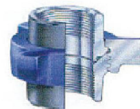
Fig 400 Hammer Union 1" - 4" 4,000 psi (276 bar) 5" - 12" 2,500 psi (172 bar) cold working pressure
