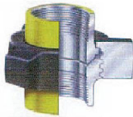
Fig 207 Hammer Union 2,000 psi (138 bar) cold working pressure
